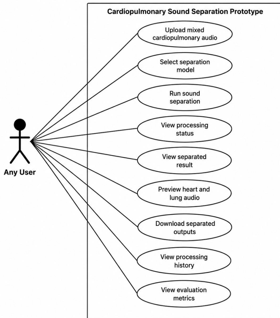
Figure 13: Use case diagram for the cardiopulmonary sound separation prototype
