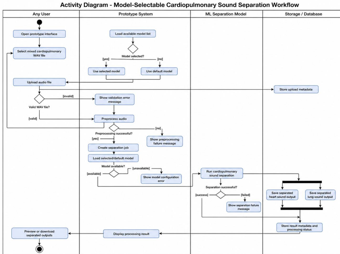
Figure 14: Activity diagram for the sound separation workflow
