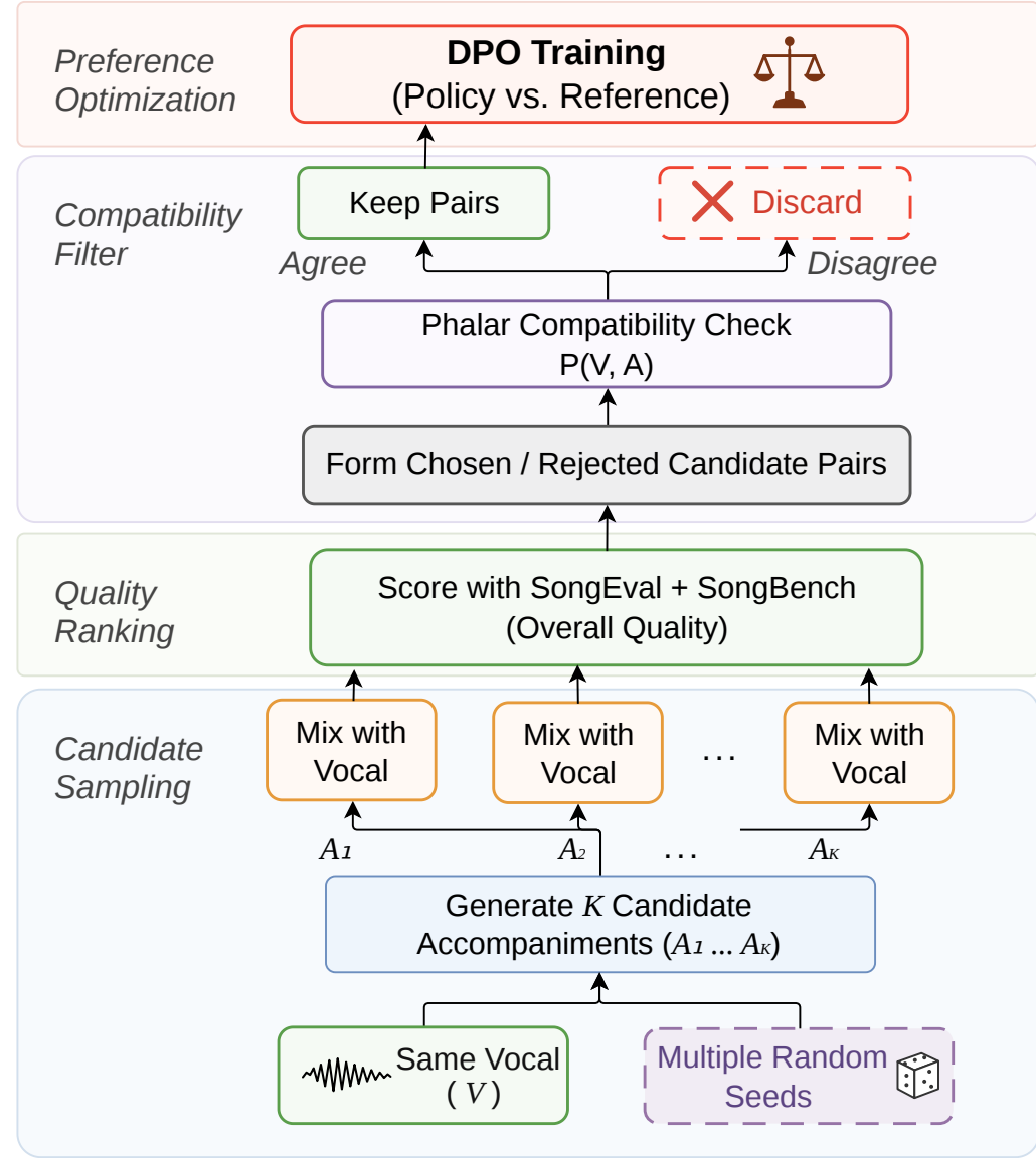
(b) Post-Training Strategy
