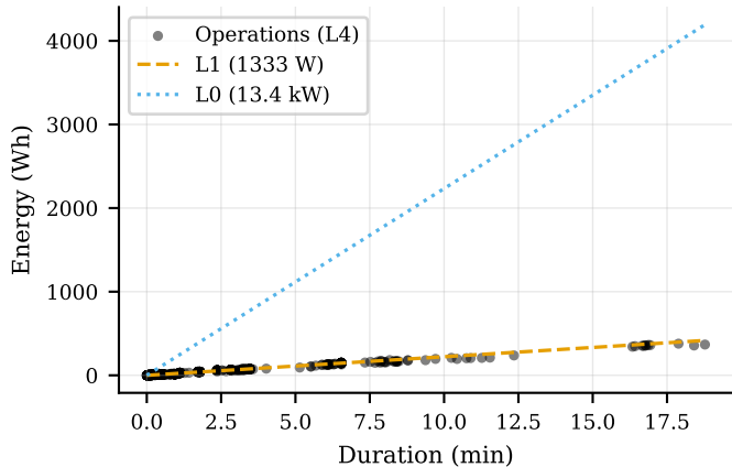
Active power (trapezoid)
