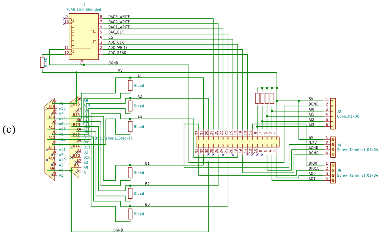
Figure 11: PCB interfacing the Control box and myRIO
