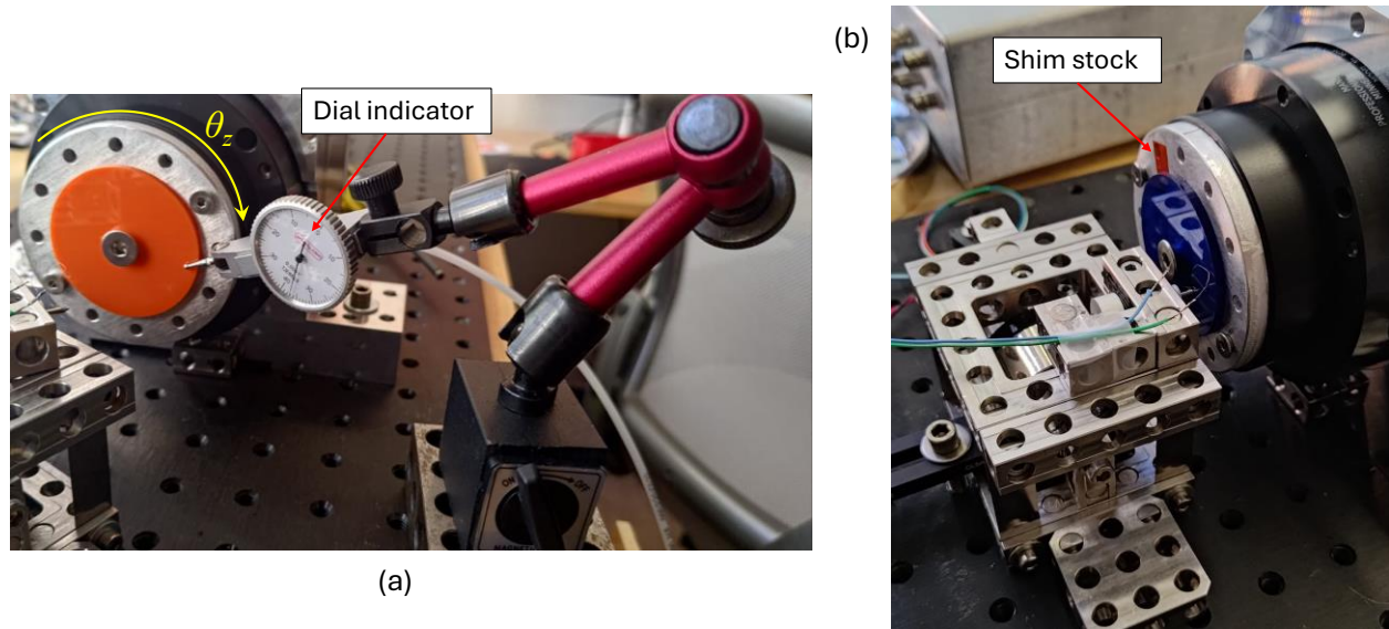
Figure 5: (a) Dial indicator to adjust the disc surface perpendicular to the spindle axis (b) by adding a shim stock under the back surface of acrylic disc.
