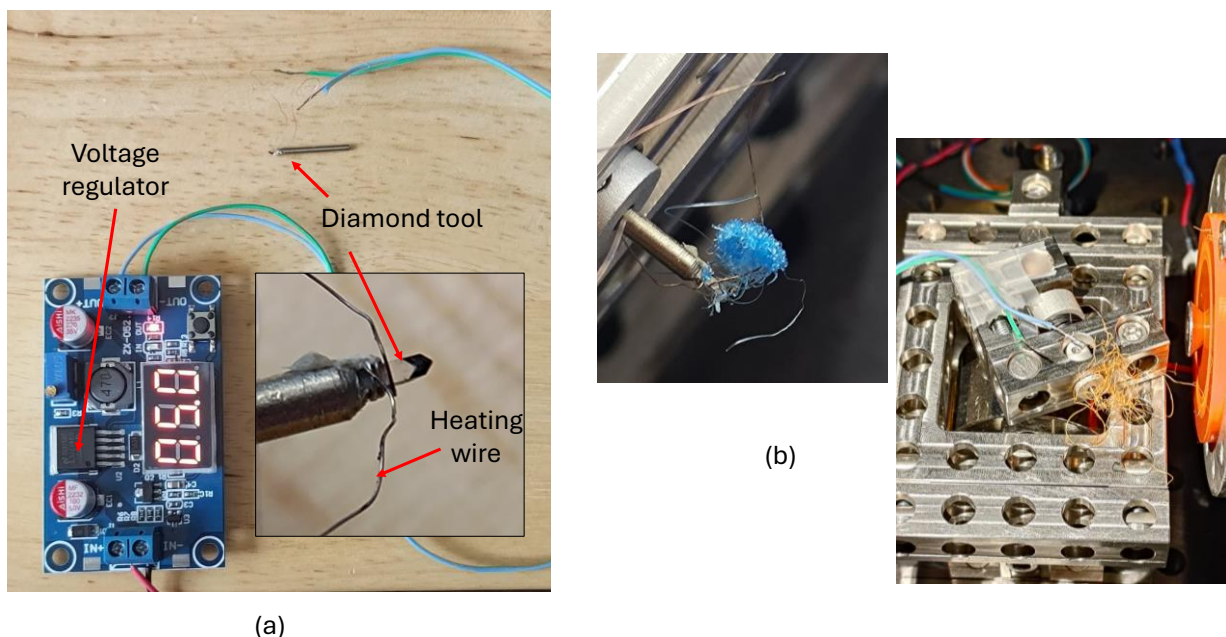
Figure 4: (a) Voltage regulator and the cutting tool with its heated wire, (b) continuous string of acrylic 'chip' that adheres to the tool.
