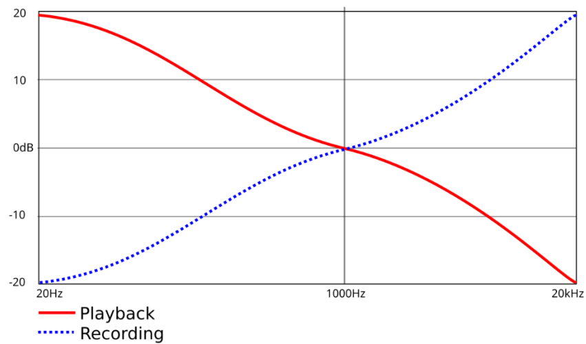
Figure 7: RIAA equalization curve
