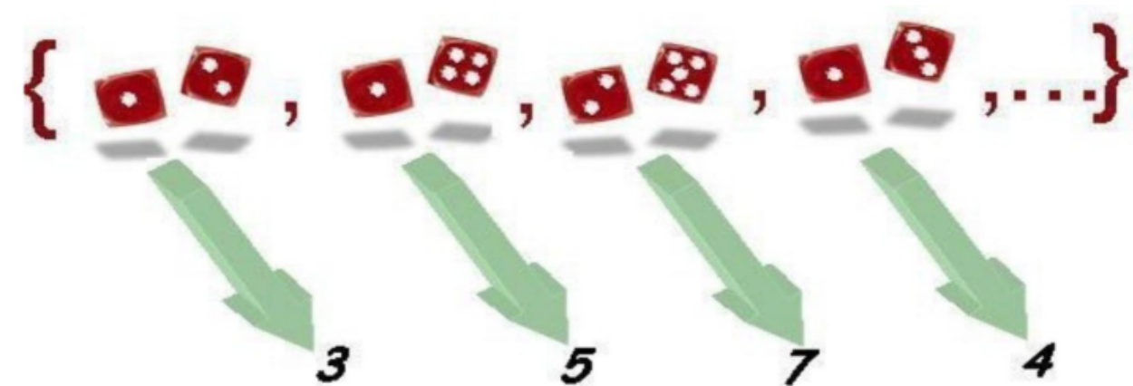
Figure 9: Recorrido de la suma.
