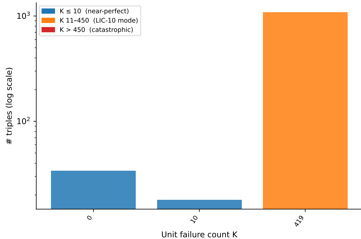
K distribution — C(20,3)=1,140 triples (trimmed) (3 unique K)
