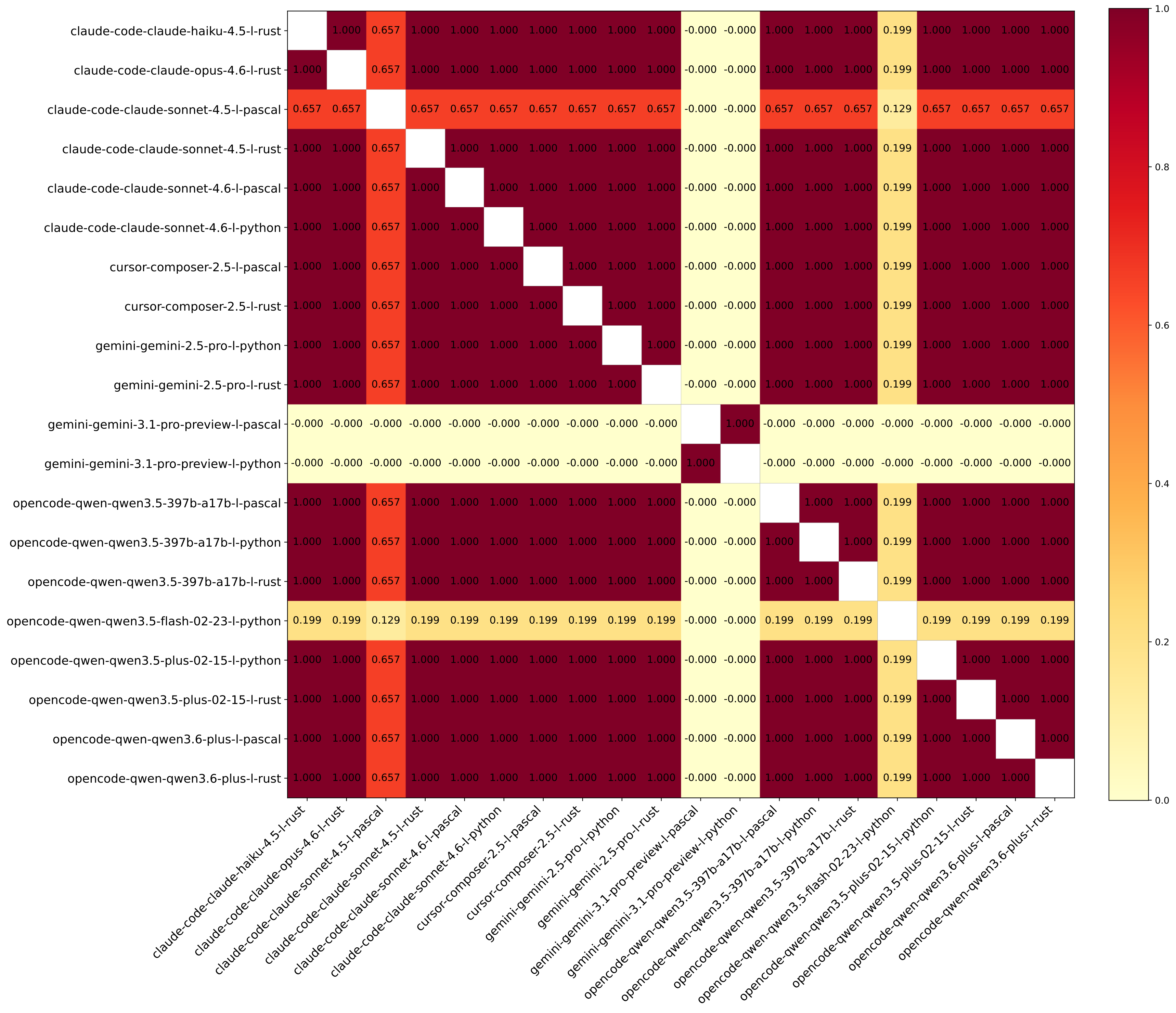
Pairwise failure analysis — Phi correlation
