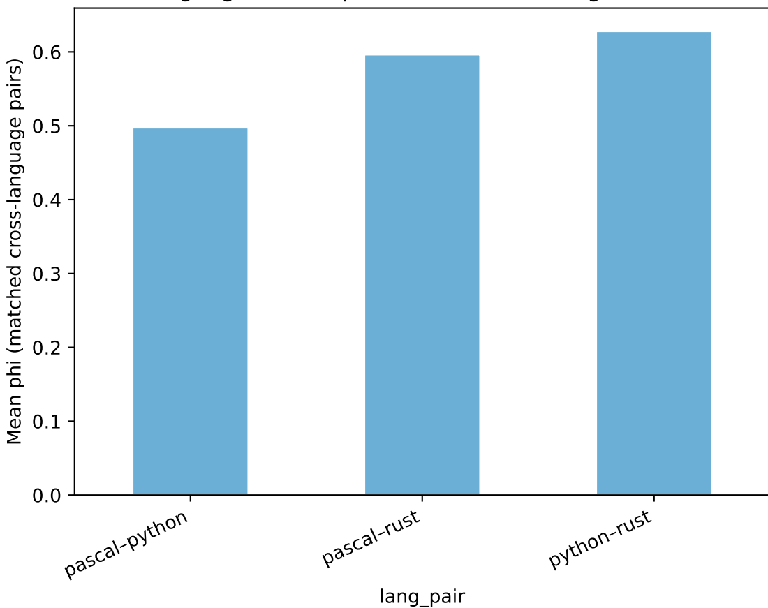
Cross-language fault dependence (matched agent/model/run)
