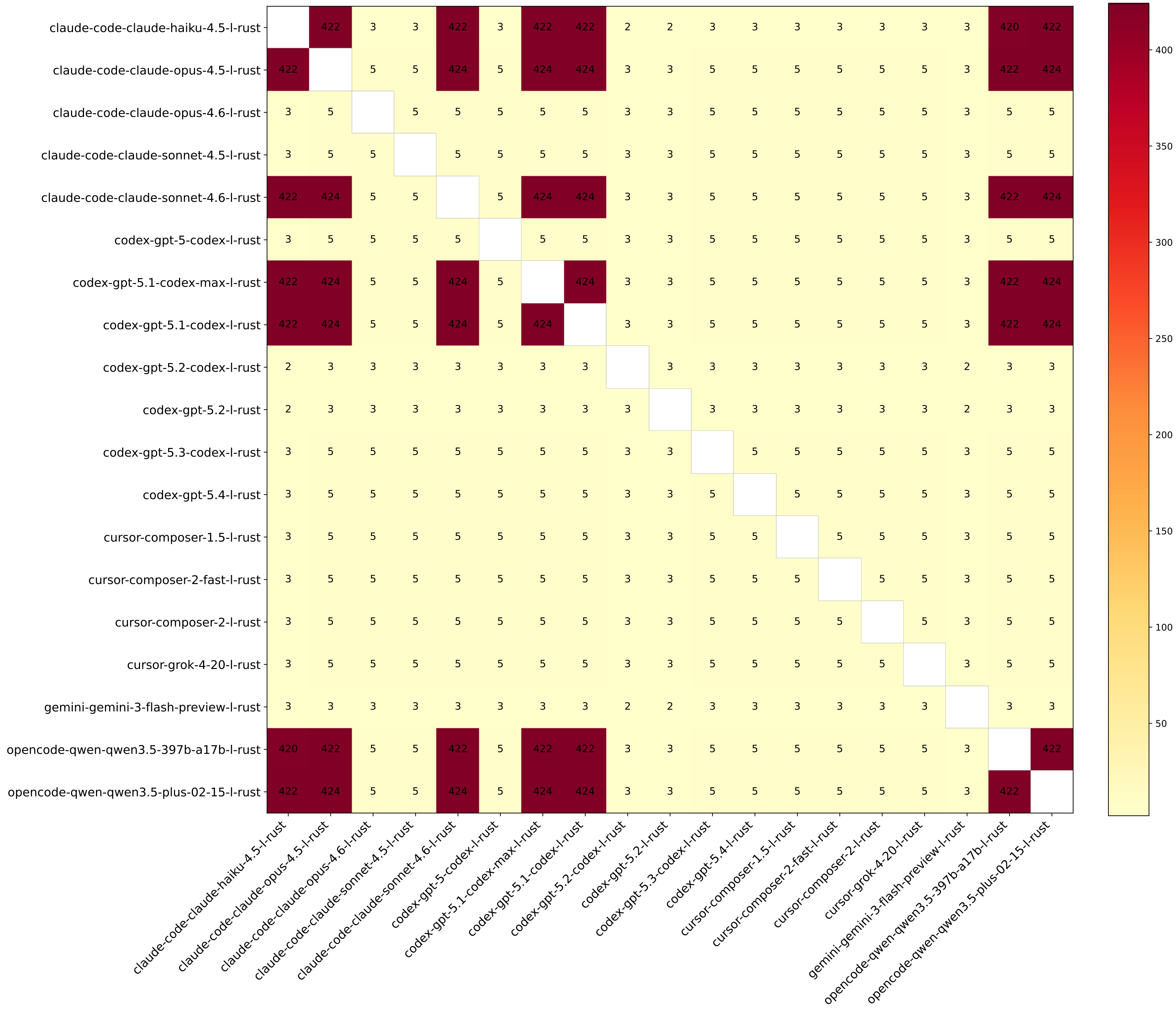
Pairwise failure analysis — Observed co-failures
