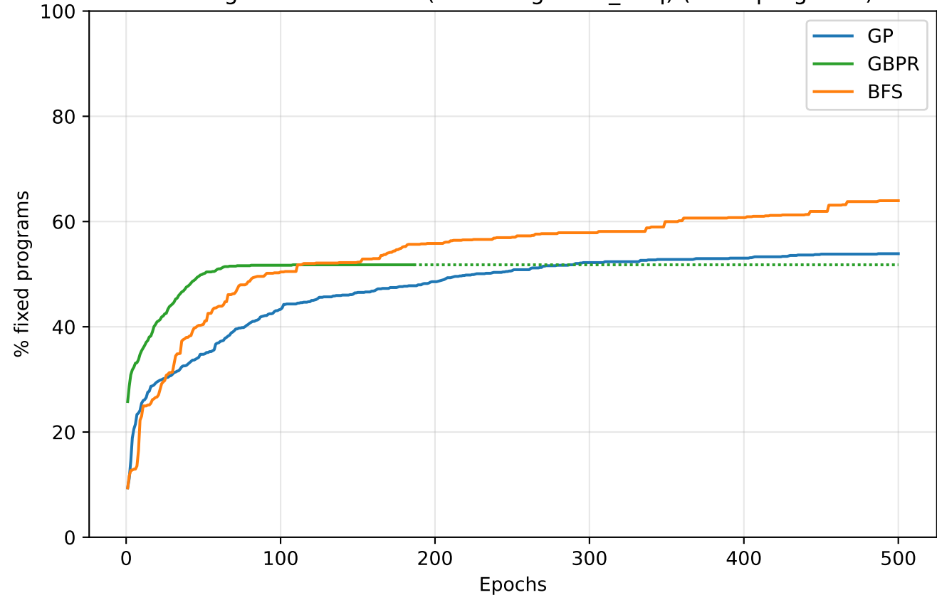
All Programs Combined (excluding most_freq) (1182 programs)
