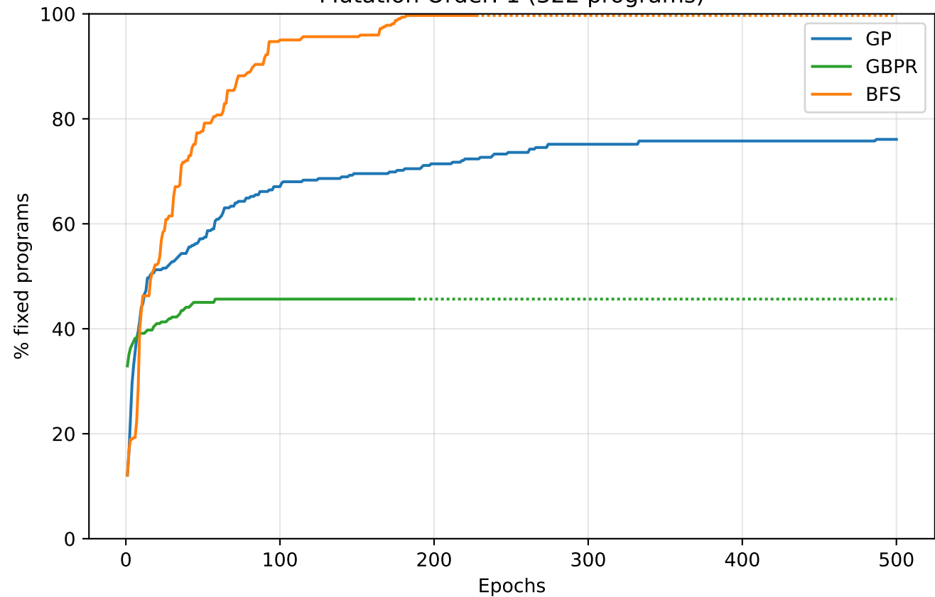
Mutation Order: 1 (322 programs)
