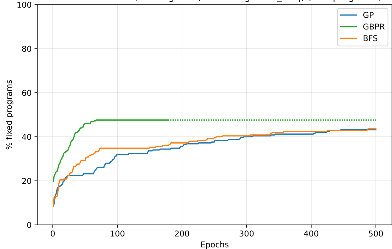
Mutation Order: 3 (All Programs, excluding most_freq) (250 programs)
