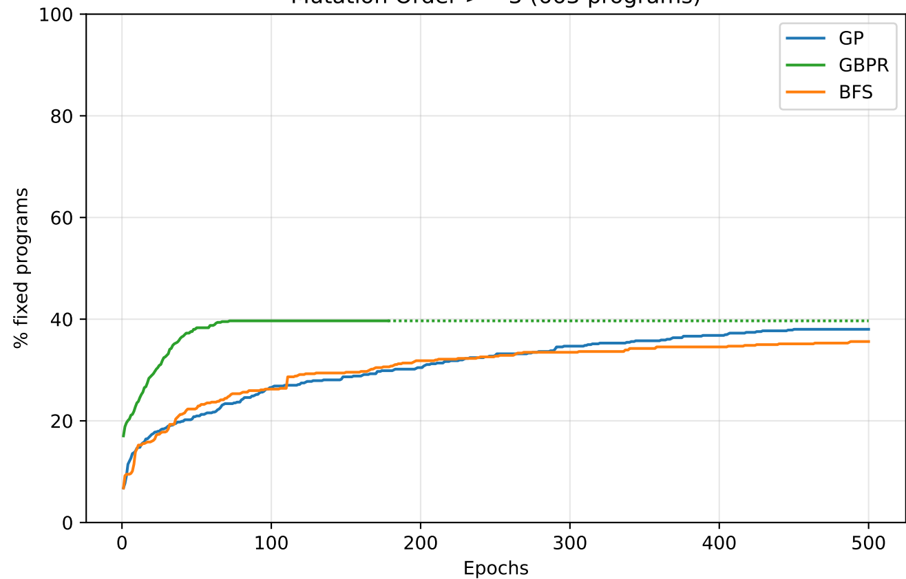
Mutation Order \geq 3 (663 programs)
