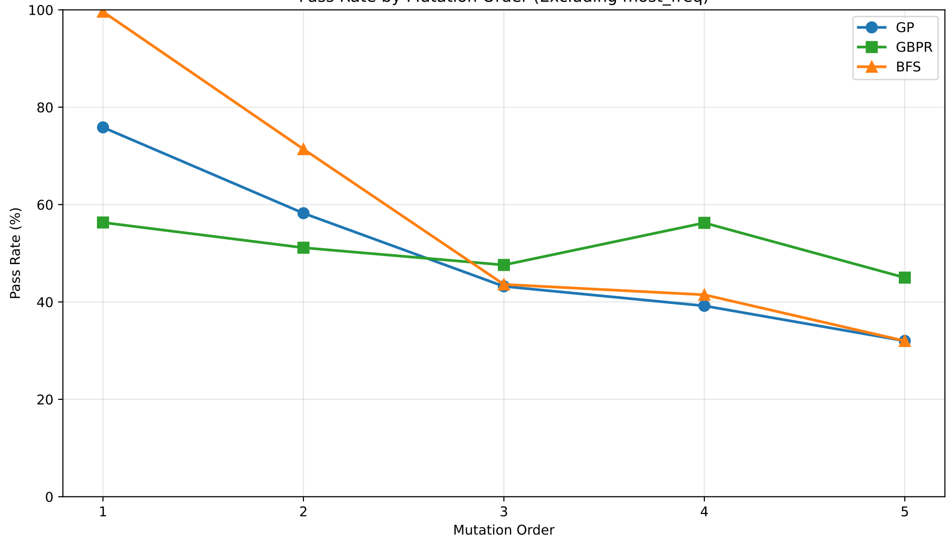
Pass Rate by Mutation Order (Excluding most_freq)
