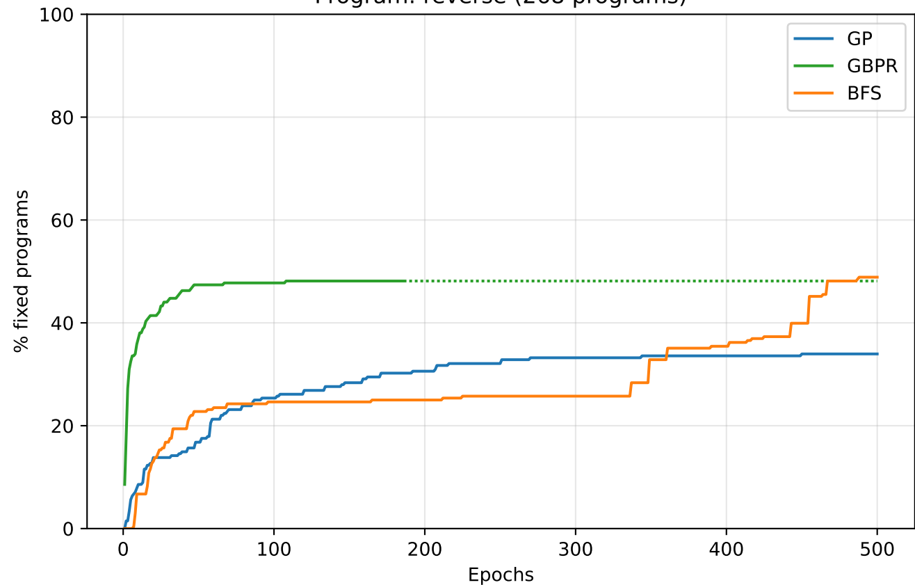
Program: reverse (268 programs)
