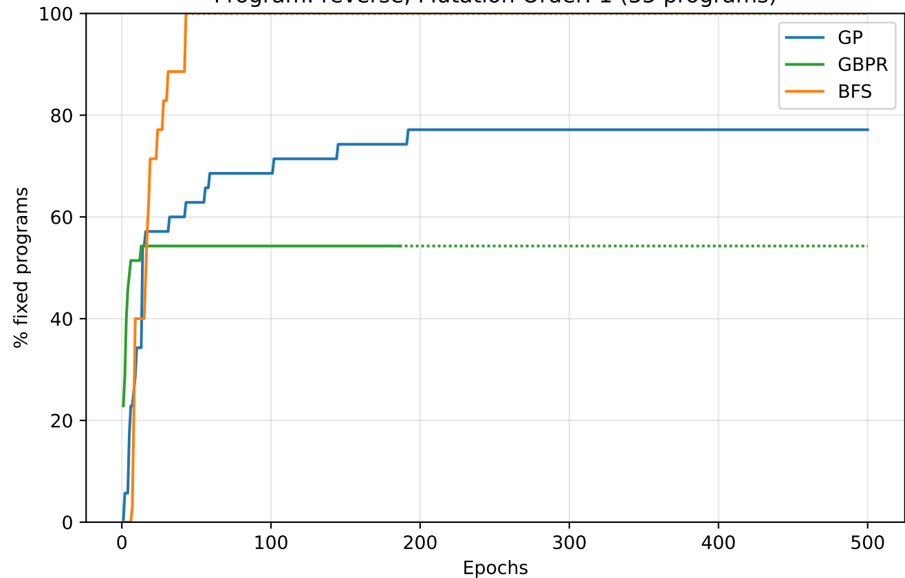
Program: reverse, Mutation Order: 1 (35 programs)
