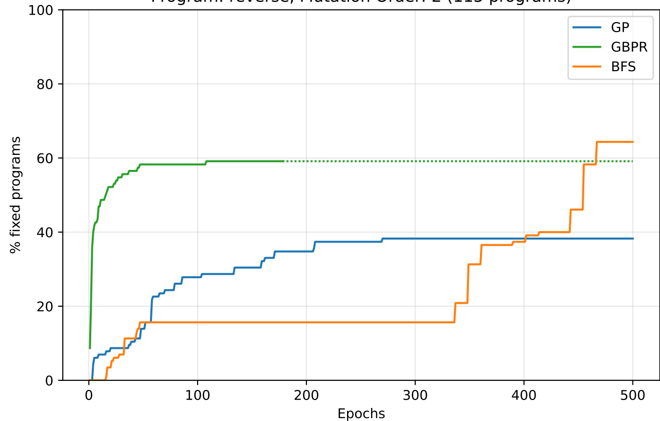
Program: reverse, Mutation Order: 2 (115 programs)
