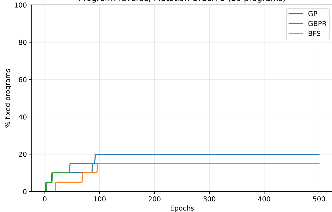
Program: reverse, Mutation Order: 5 (20 programs)
