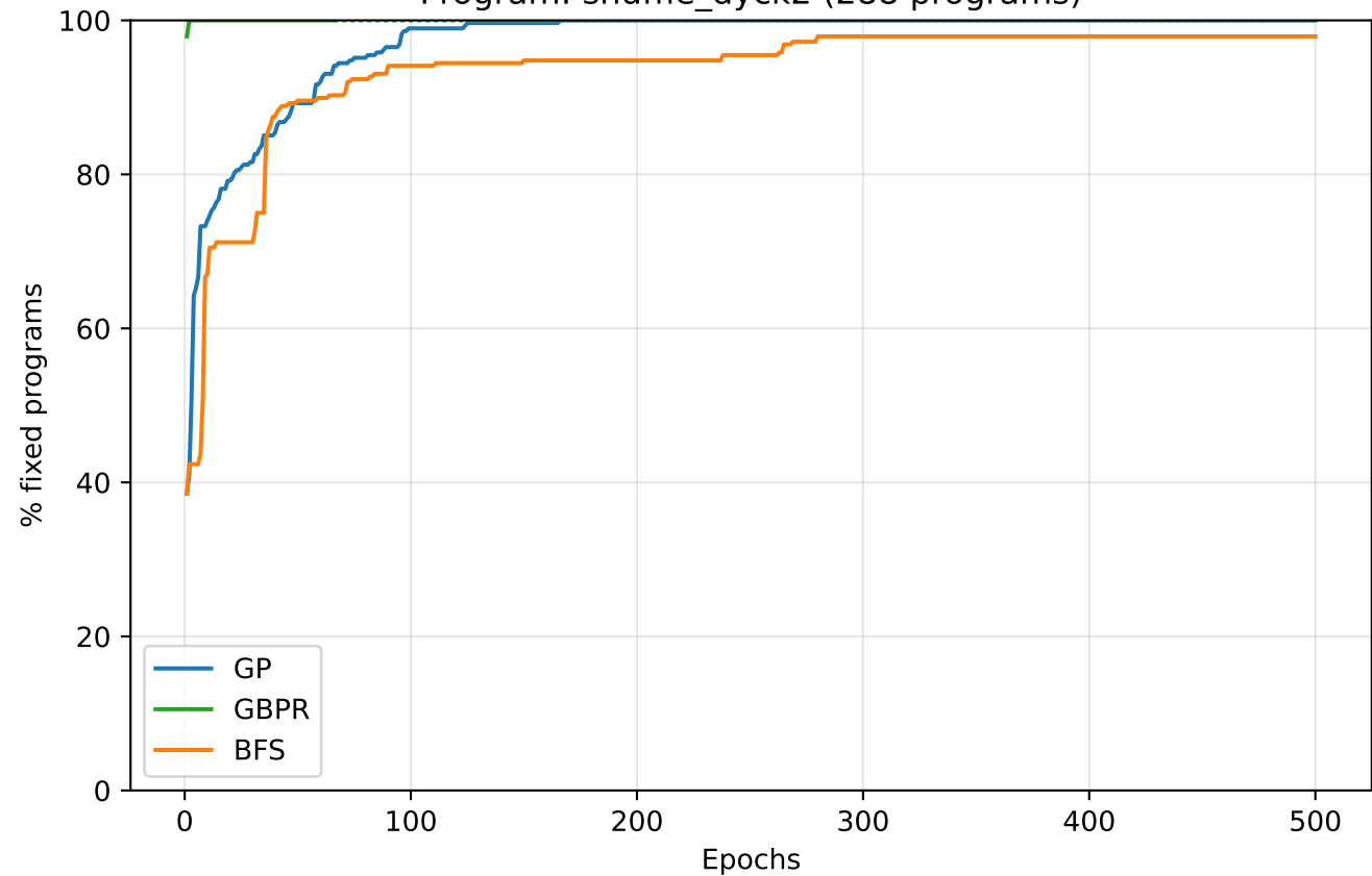
Program: shuffle_dyck2 (288 programs)
