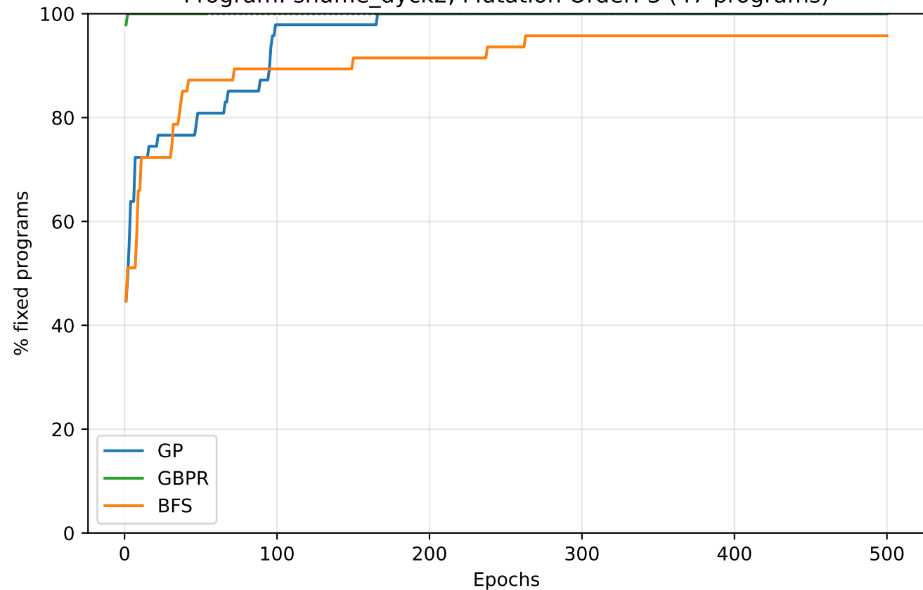
Program: shuffle_dyck2, Mutation Order: 3 (47 programs)
