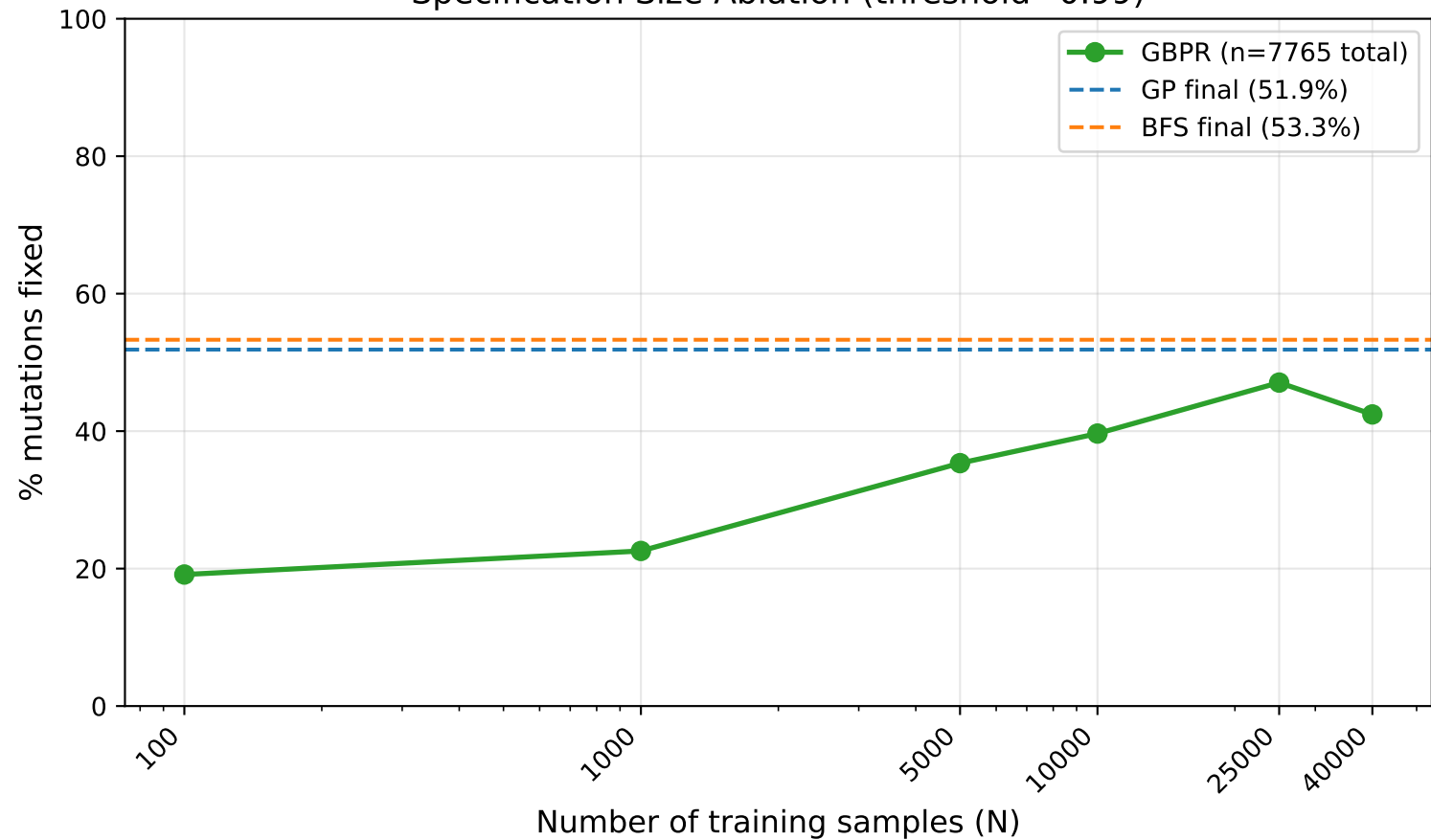
Specification Size Ablation (threshold=0.99)
