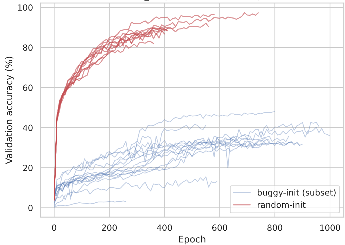
most_freq: validation accuracy
