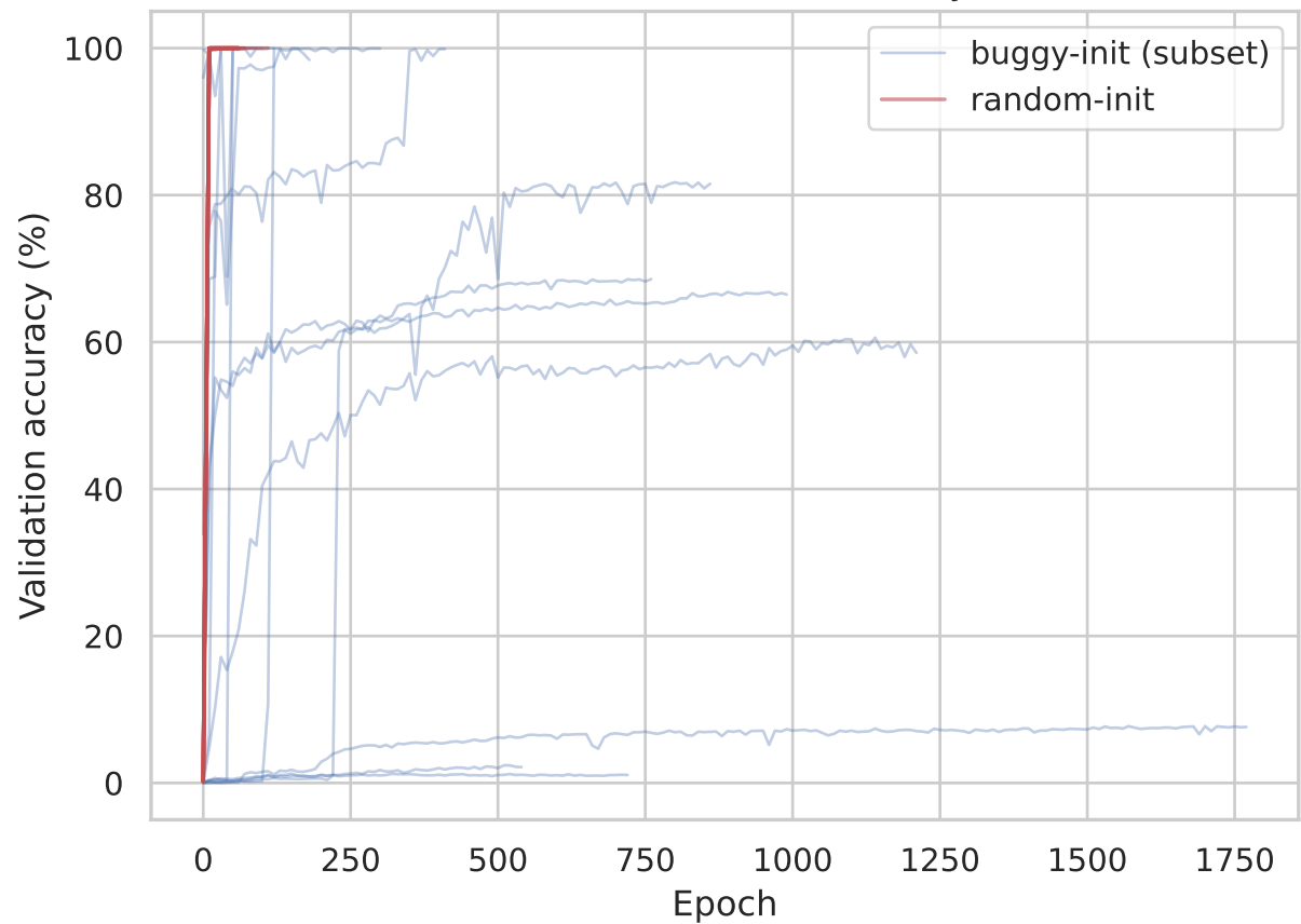
reverse: validation accuracy
