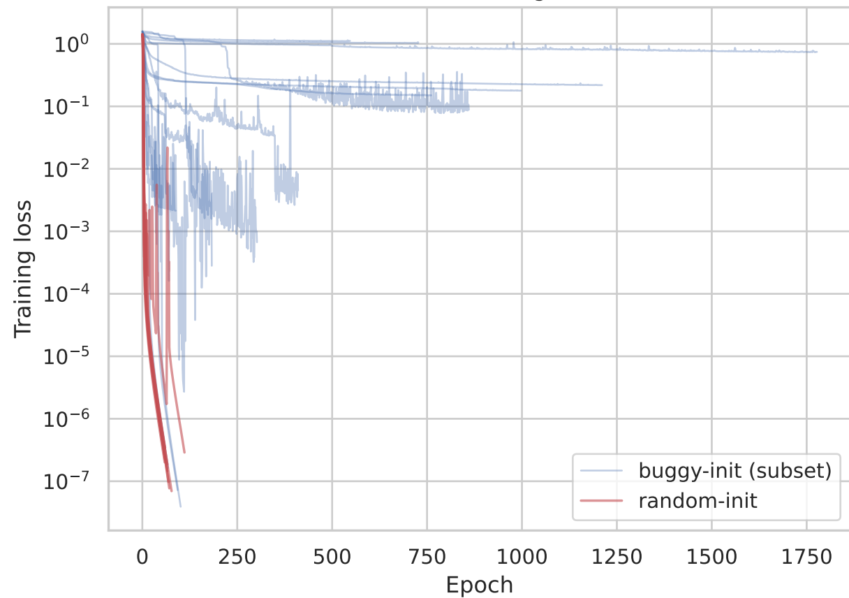
reverse: training loss
