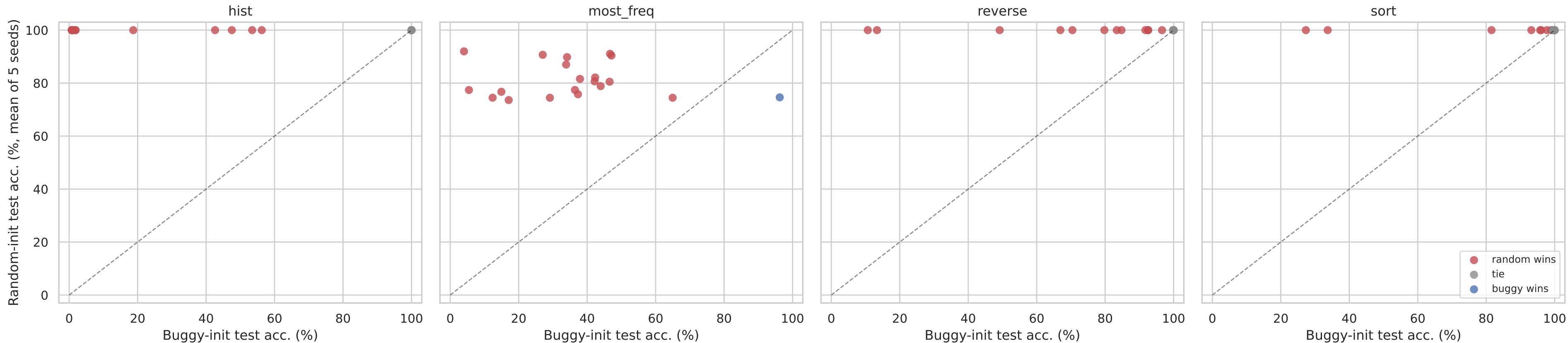
Paired initialization control: same mutant architecture, buggy vs. random weights
