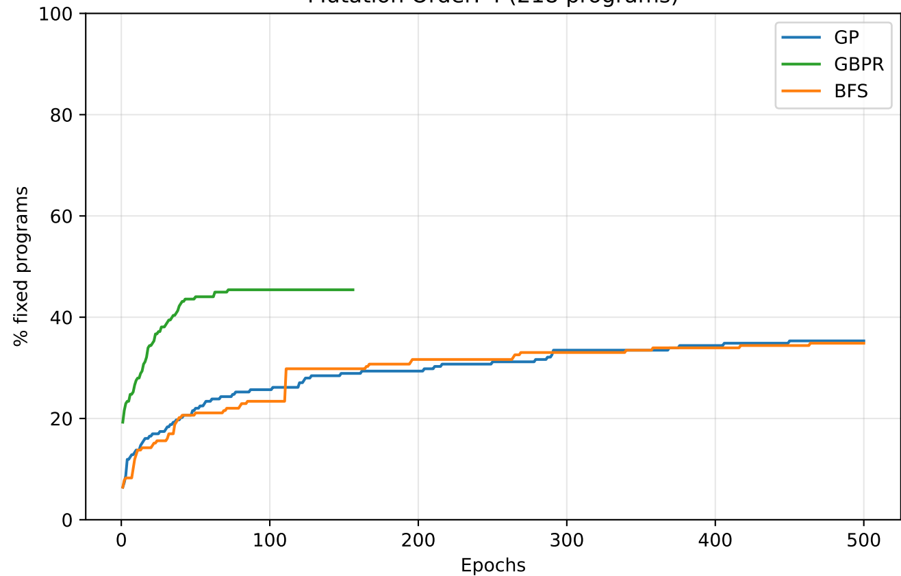
Mutation Order: 4 (218 programs)
