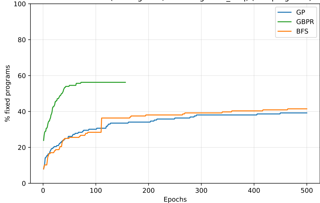
Mutation Order: 4 (All Programs, excluding most_freq) (176 programs)
