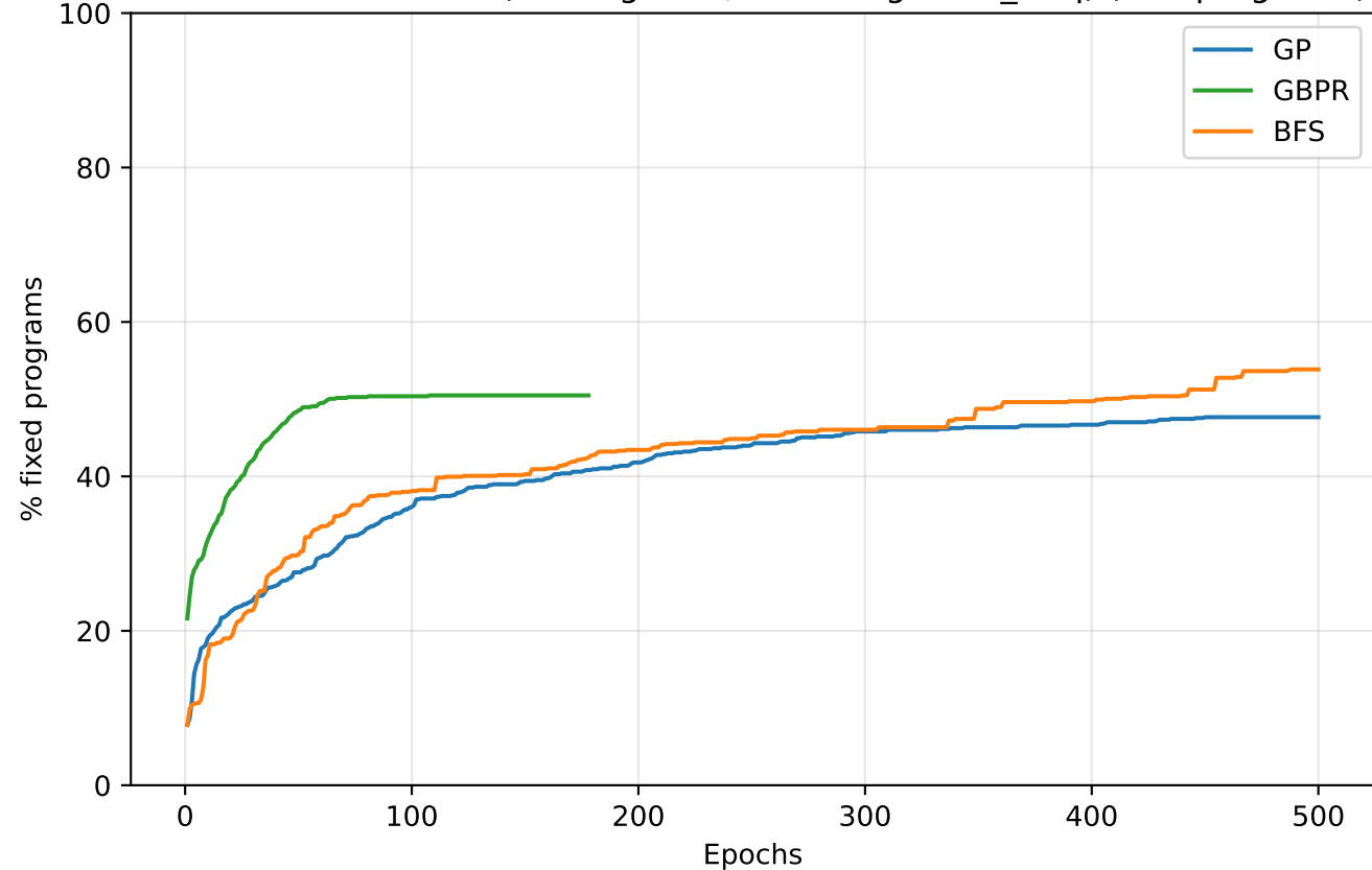
Mutation Order \geq 2 (All Programs, excluding most_freq) (921 programs)
