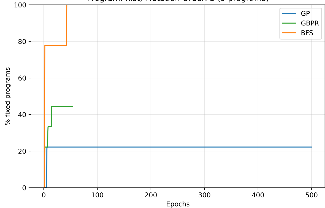
Program: hist, Mutation Order: 3 (9 programs)
