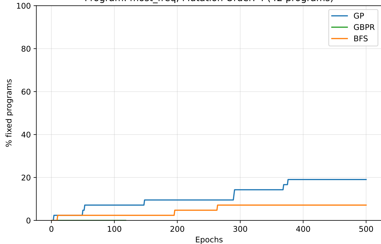
Program: most_freq, Mutation Order: 4 (42 programs)
