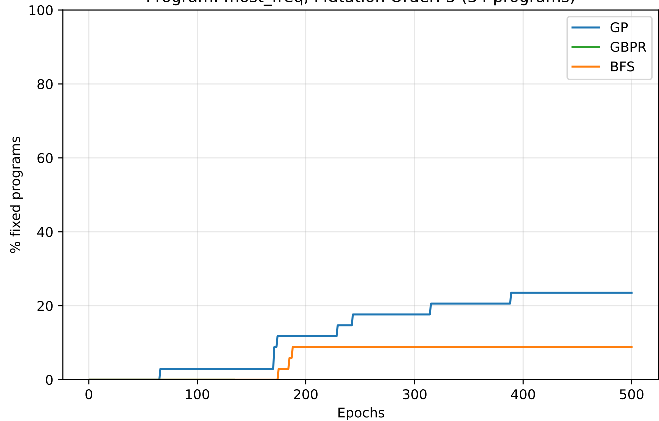
Program: most_freq, Mutation Order: 5 (34 programs)
