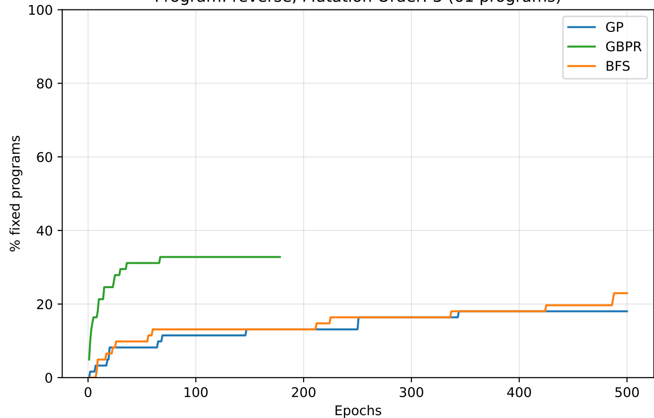
Program: reverse, Mutation Order: 3 (61 programs)
