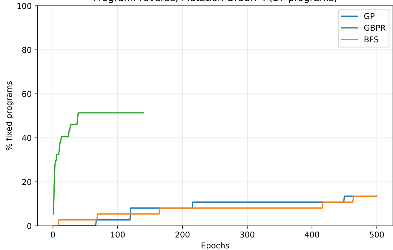
Program: reverse, Mutation Order: 4 (37 programs)
