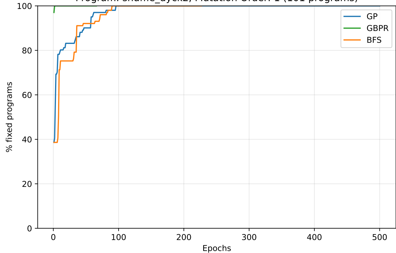
Program: shuffle_dyck2, Mutation Order: 1 (101 programs)
