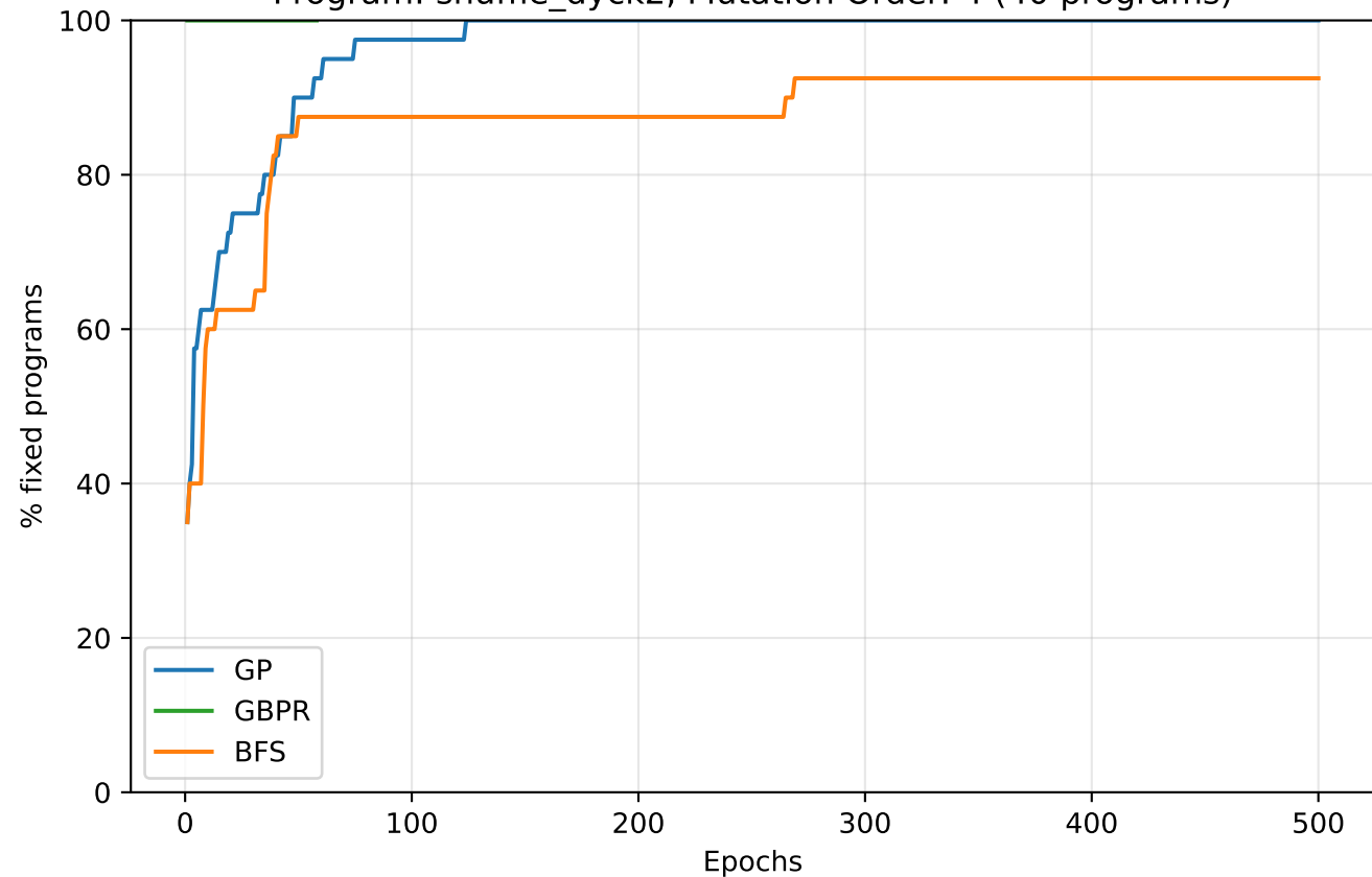
Program: shuffle_dyck2, Mutation Order: 4 (40 programs)
