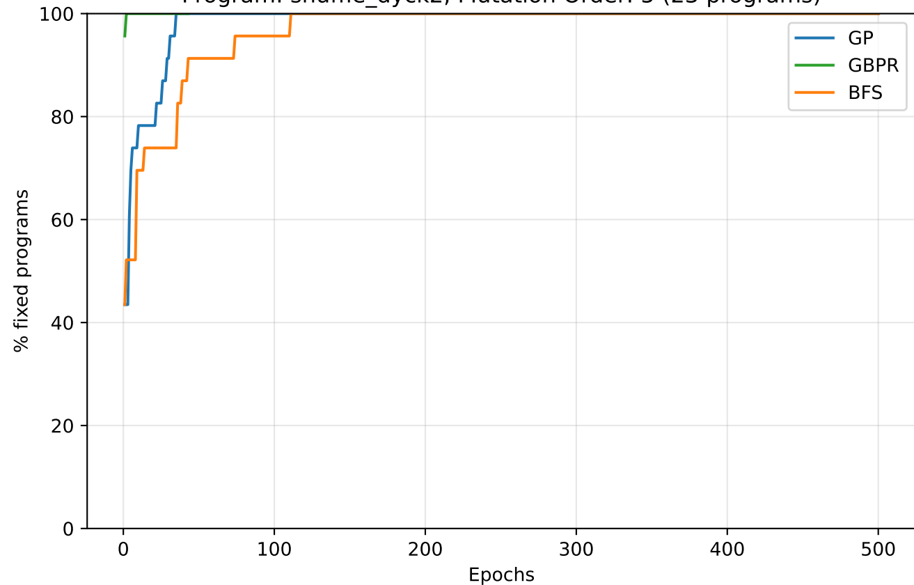
Program: shuffle_dyck2, Mutation Order: 5 (23 programs)
