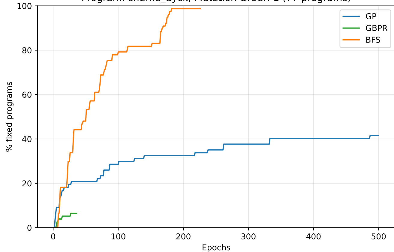
Program: shuffle_dyck, Mutation Order: 1 (77 programs)
