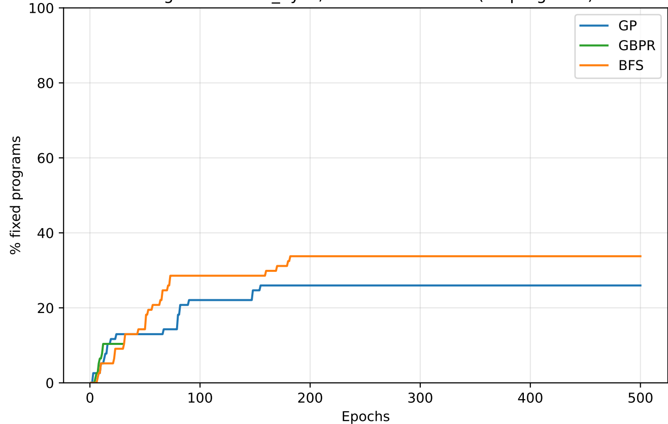
Program: shuffle_dyck, Mutation Order: 3 (77 programs)
