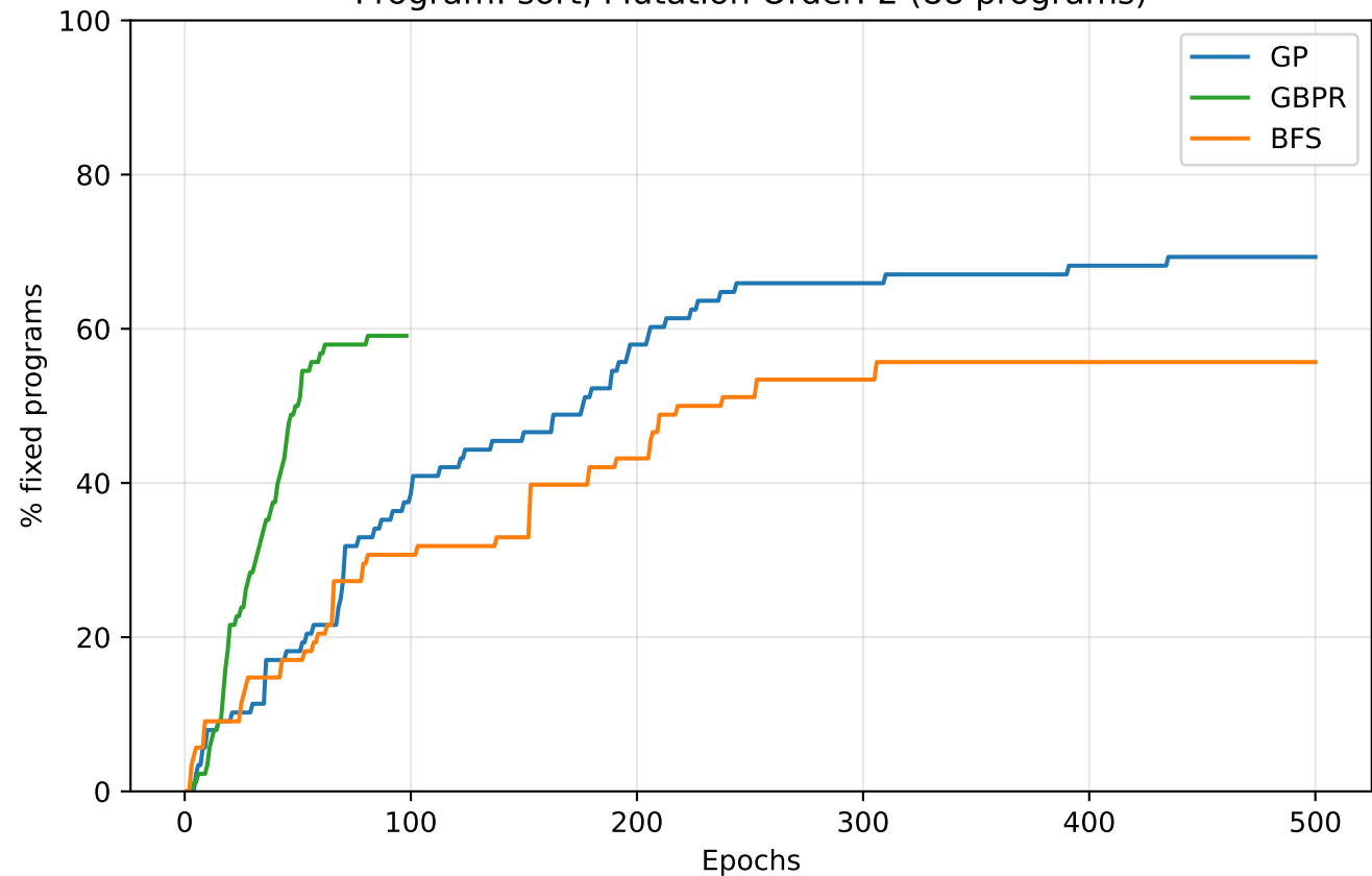
Program: sort, Mutation Order: 2 (88 programs)
