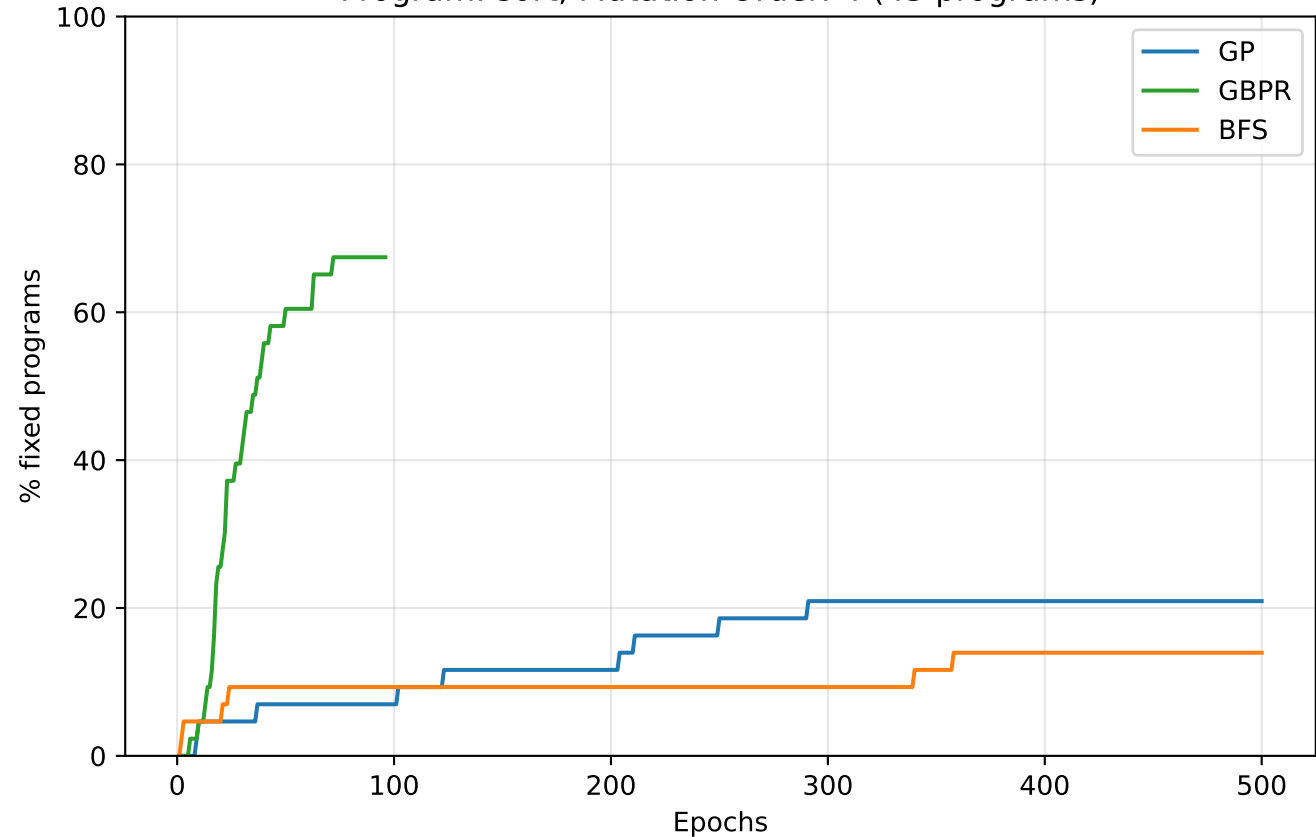
Program: sort, Mutation Order: 4 (43 programs)
