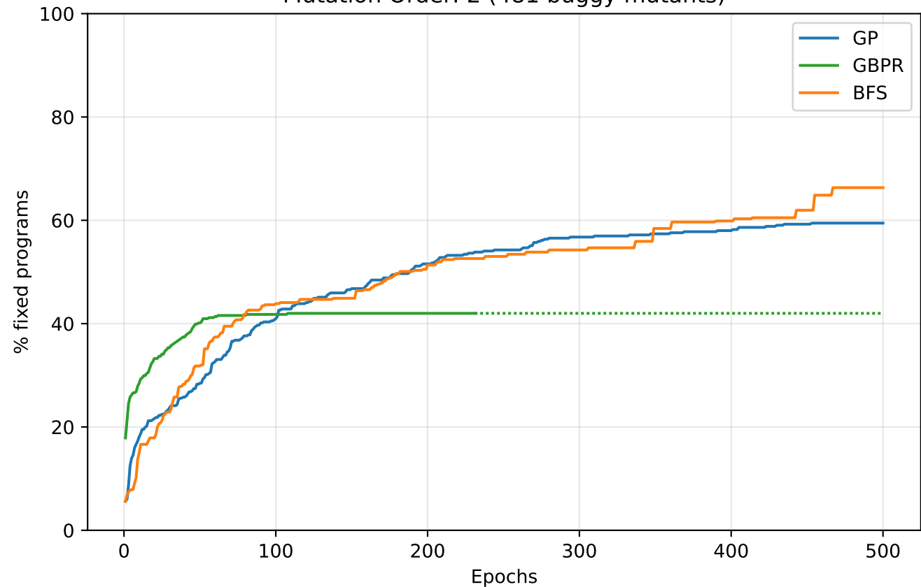
Mutation Order: 2 (481 buggy mutants)
