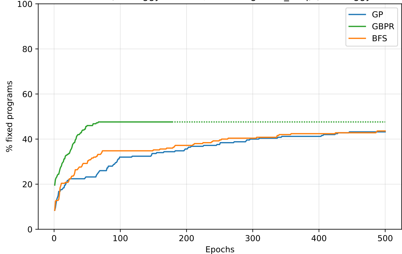
Mutation Order: 3 (All Buggy Mutants, excluding most_freq) (250 buggy mutants)
