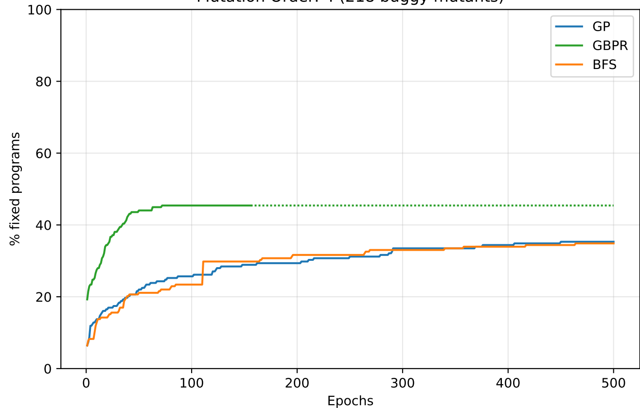
Mutation Order: 4 (218 buggy mutants)
