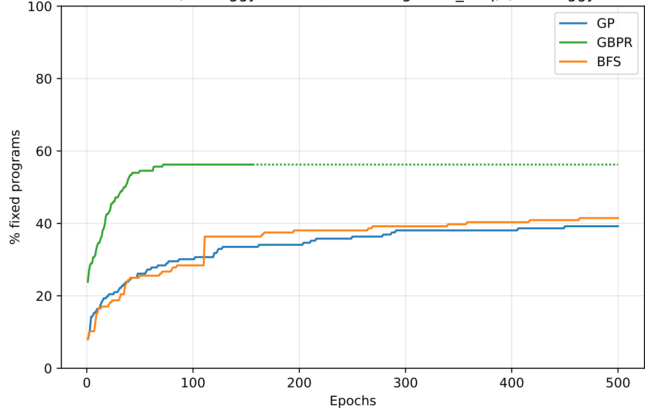
Mutation Order: 4 (All Buggy Mutants, excluding most_freq) (176 buggy mutants)
