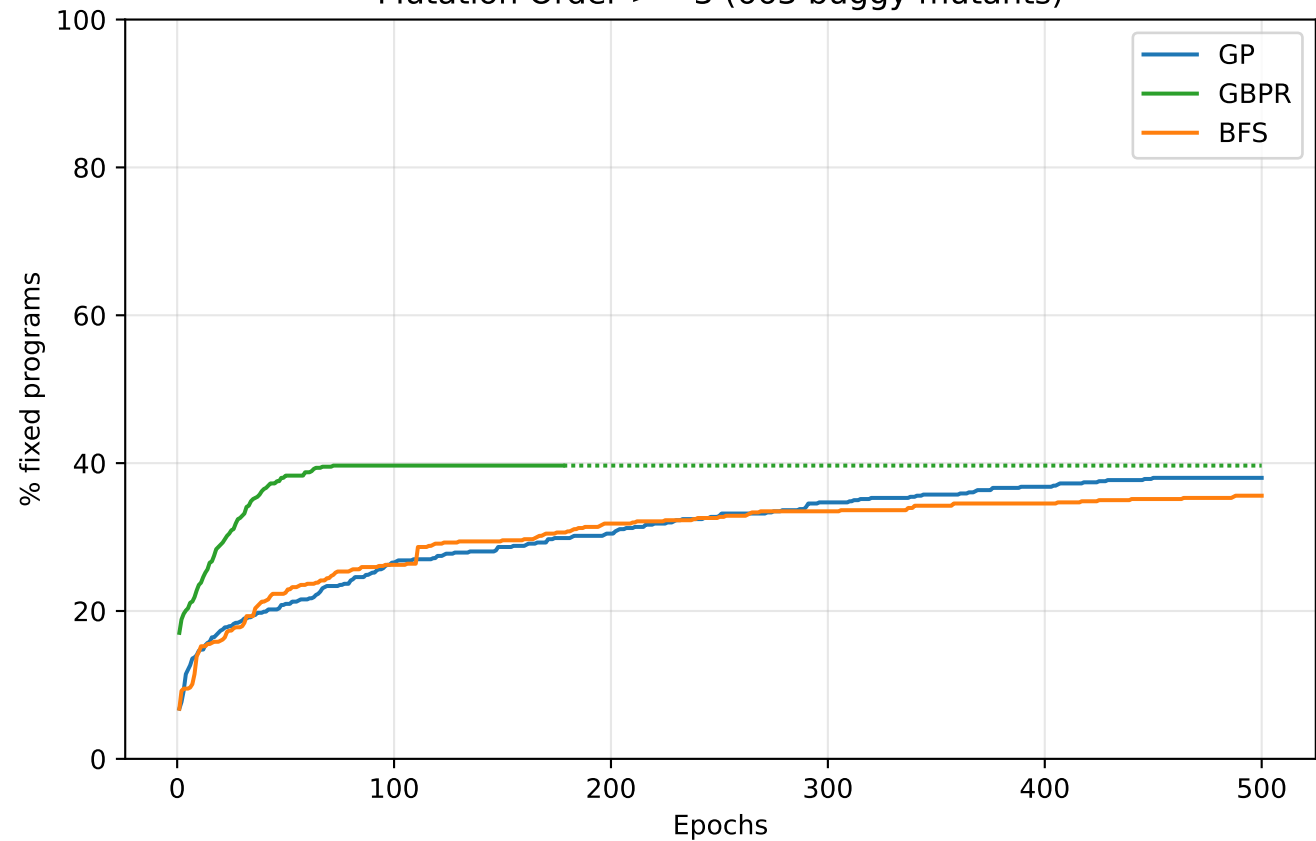
Mutation Order \geq 3 (663 buggy mutants)
