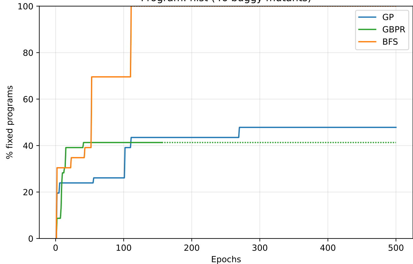
Program: hist (46 buggy mutants)
