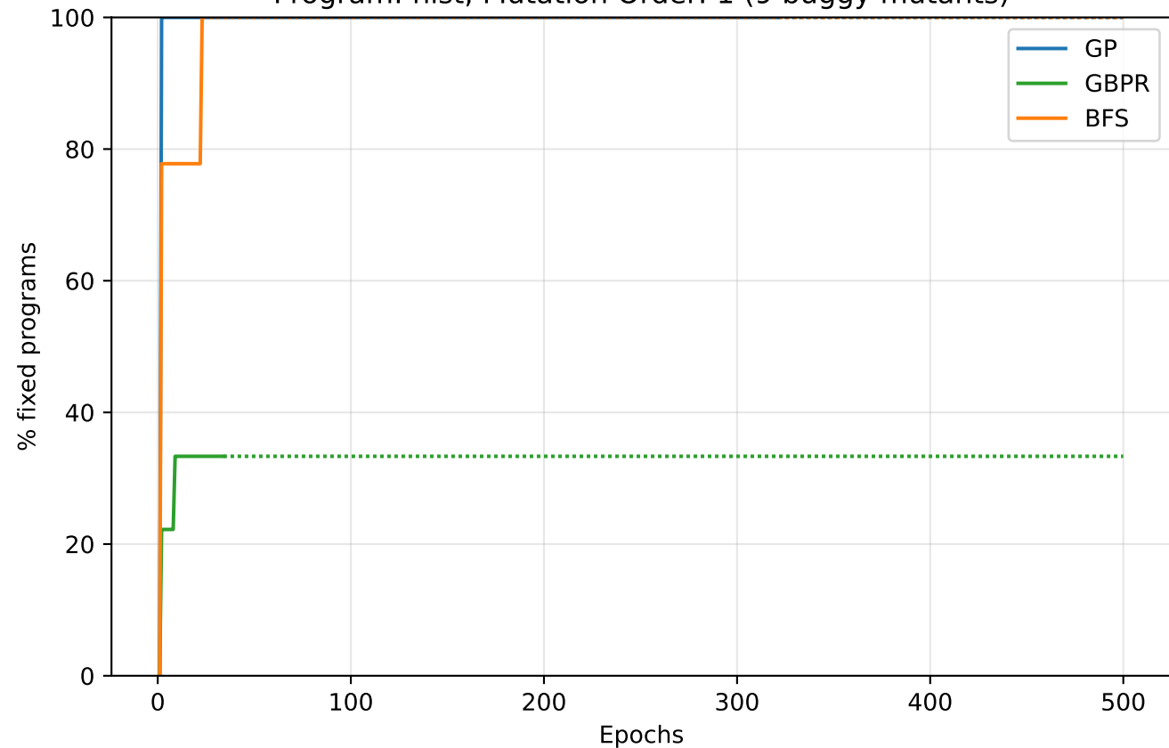
Program: hist, Mutation Order: 1 (9 buggy mutants)
