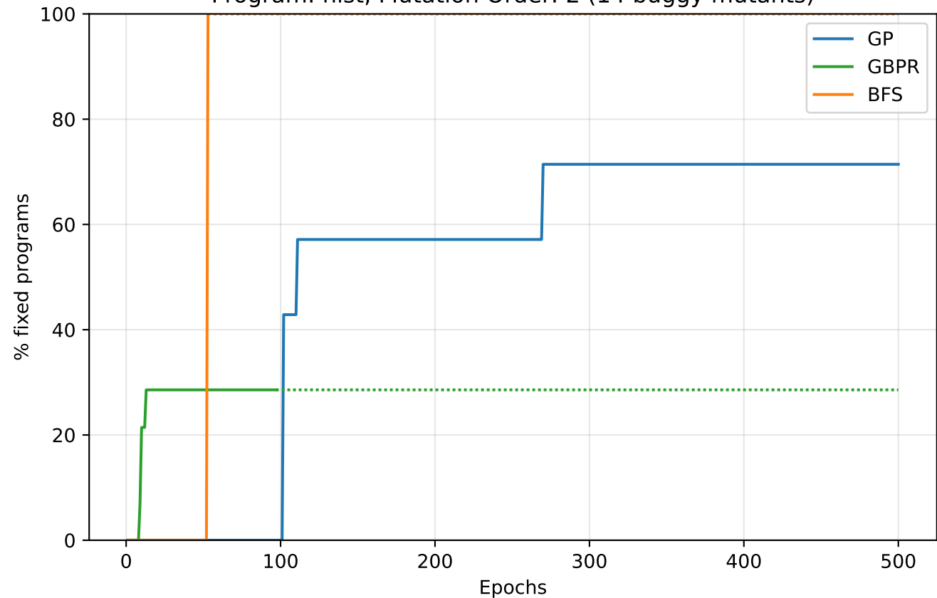
Program: hist, Mutation Order: 2 (14 buggy mutants)
