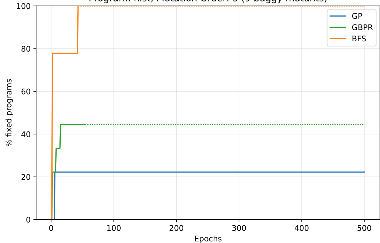
Program: hist, Mutation Order: 3 (9 buggy mutants)
