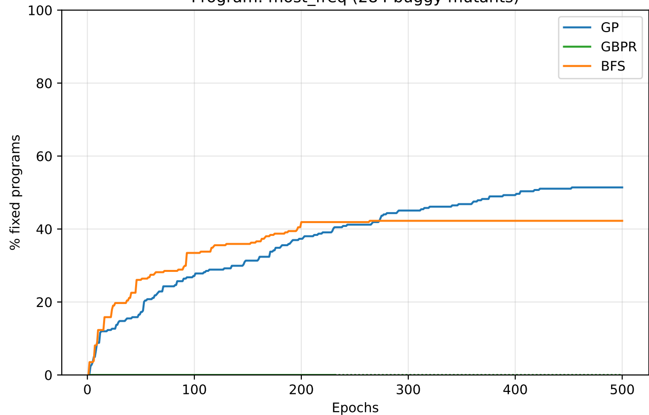
Program: most_freq (284 buggy mutants)
