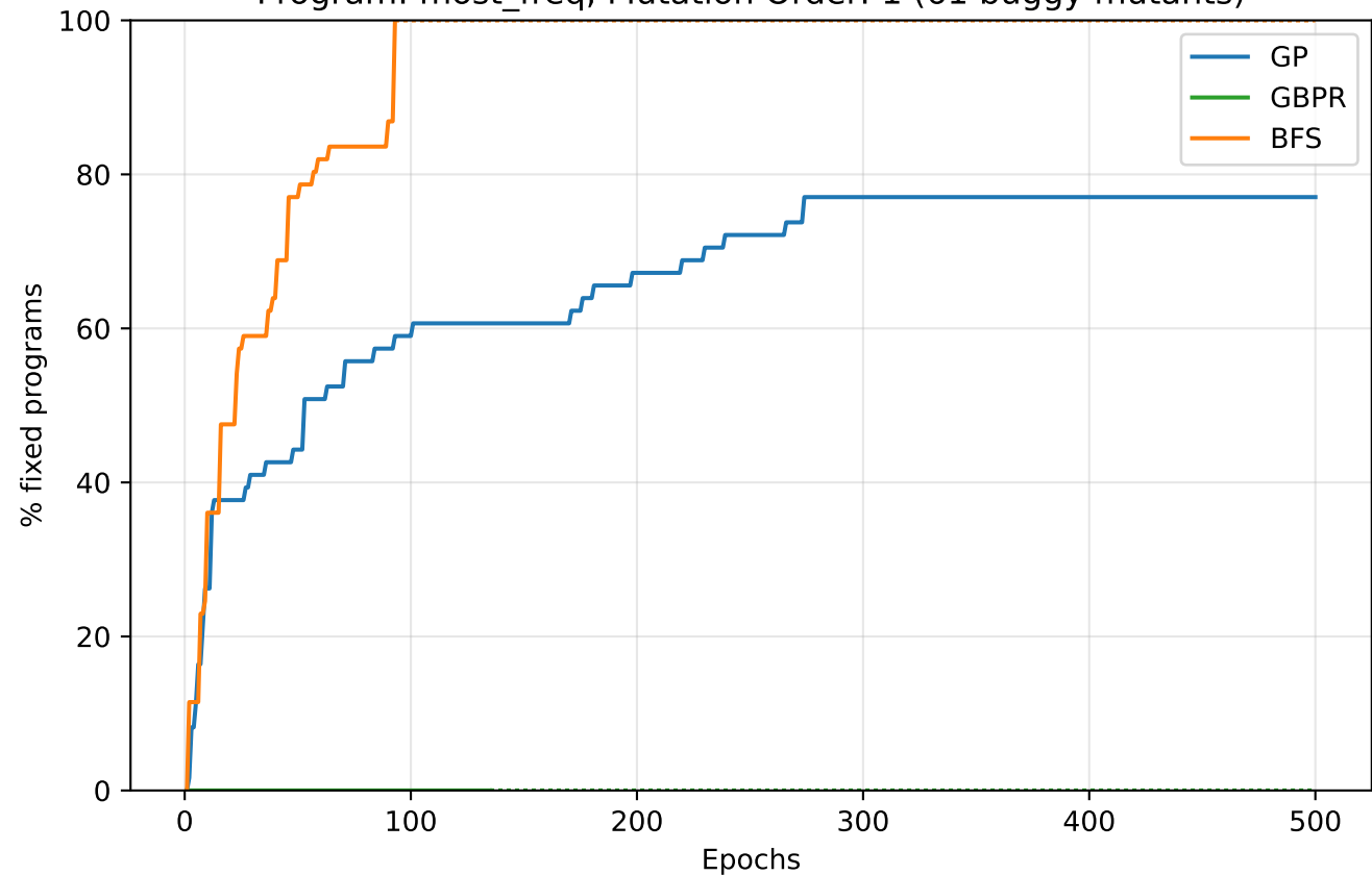
Program: most_freq, Mutation Order: 1 (61 buggy mutants)
